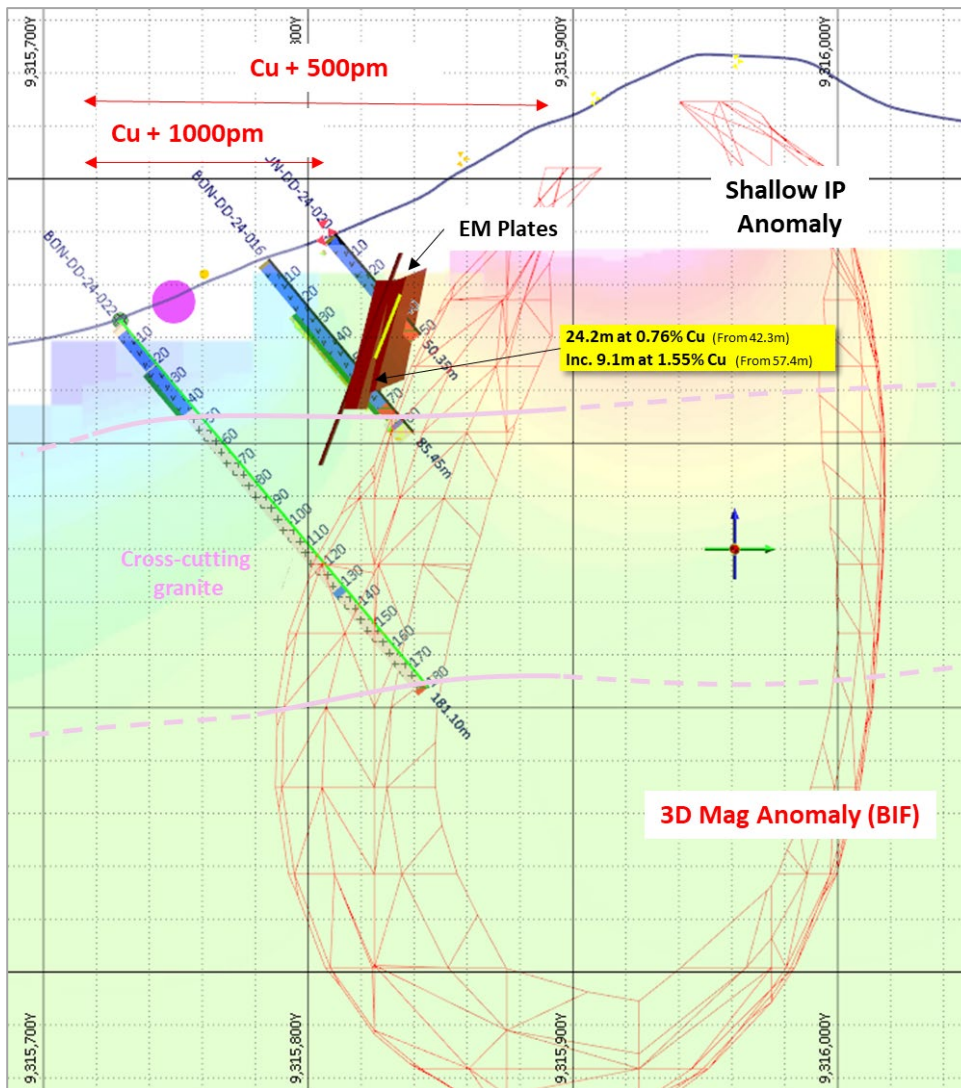
Figure 2 – Nelore West Prospect – Section 657450mE.
