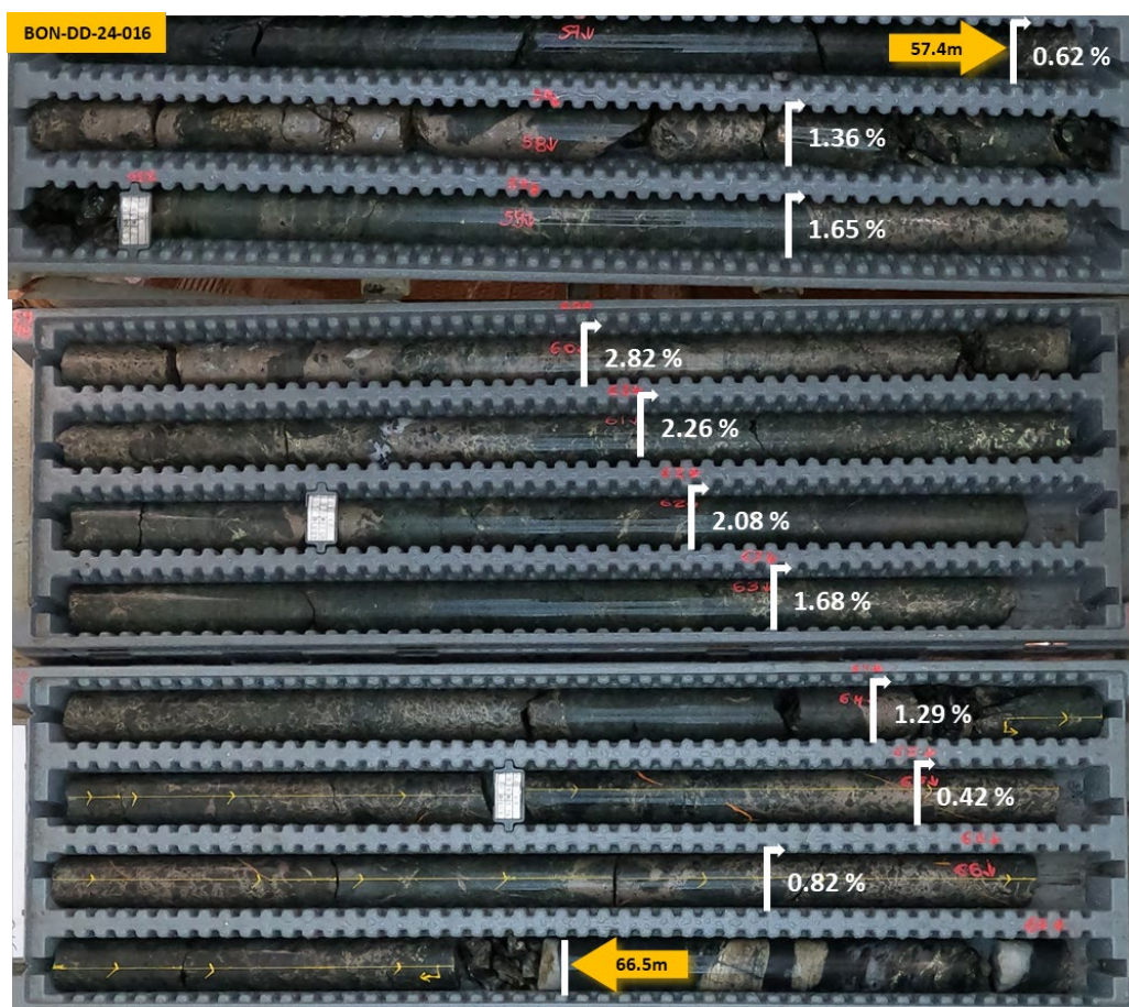
Figure 1 – Nelore West Prospect – core photo from drill-hole BON-DD-24-016 Stringer and semi-massive sulphides – pyrrhotite (brown-bronze colour) >> chalcopyrite (brassy yellow) > pyrite. Assays returned 9.1m at 1.55% Cu and 0.08ppm Au from 57.4m.
